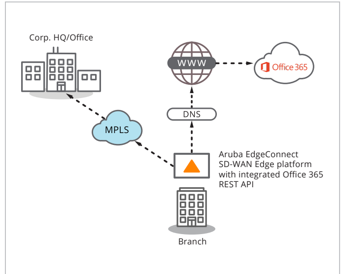
Figure 10: EdgeConnect enables secure internet breakout directly from the branch office to the closest Office 365 entry point using the latest Office 365 endpoint data.
