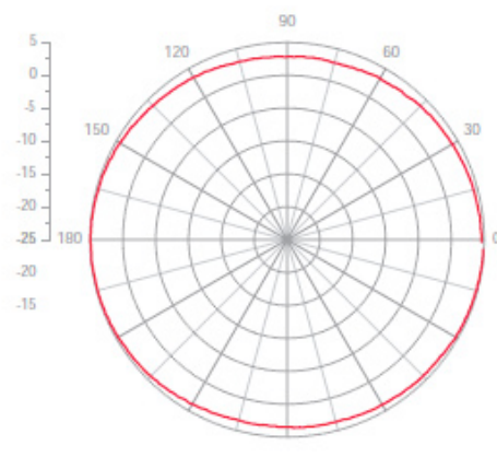
5750 MHz
