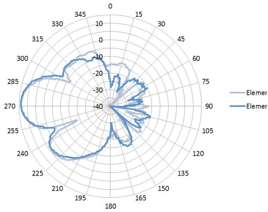
E-plane (side view) - 2.46 GHz
