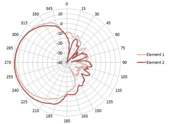
H-plane (top view) - 2.46 GHz
