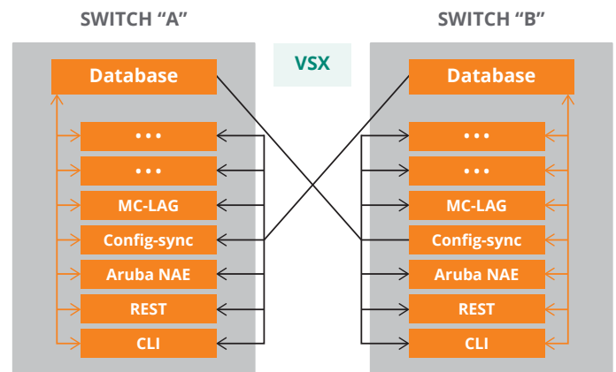
Figure 4: The Aruba VSX provides a redundant architecture that is highly available with minimal to zero traffic loss, even during live upgrades of software.
